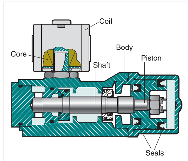
Four-way valves use four or five pipe connections – one pressure, two cylinder, one or two exhaust – to operate double-acting cylinders or actuators.
