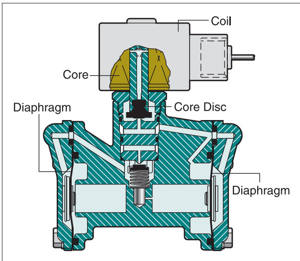
Three-way valves have three connections and two orifices and are available as normally open, normally closed, or universal, whereby they can be employed as either normally open or normally closed.
