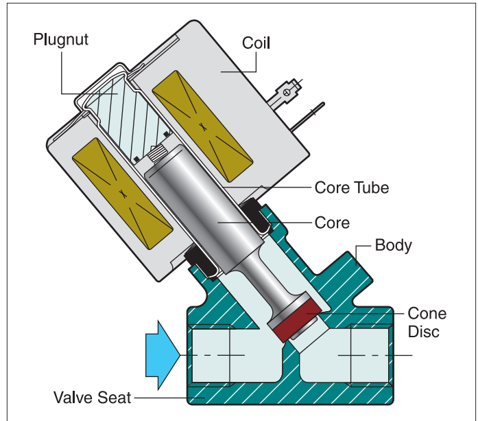
Two-way solenoid valves have one inlet and one outlet pipe connection and are not bidirectional. They are suitable for flow in one direction only.
